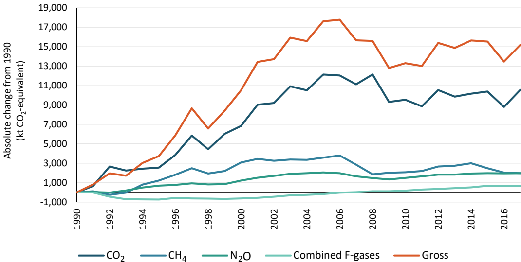
Figure 1.4: Change in New Zealand’s gross emissions by gas 1990–2017 (using 1990 emissions as a base level)
